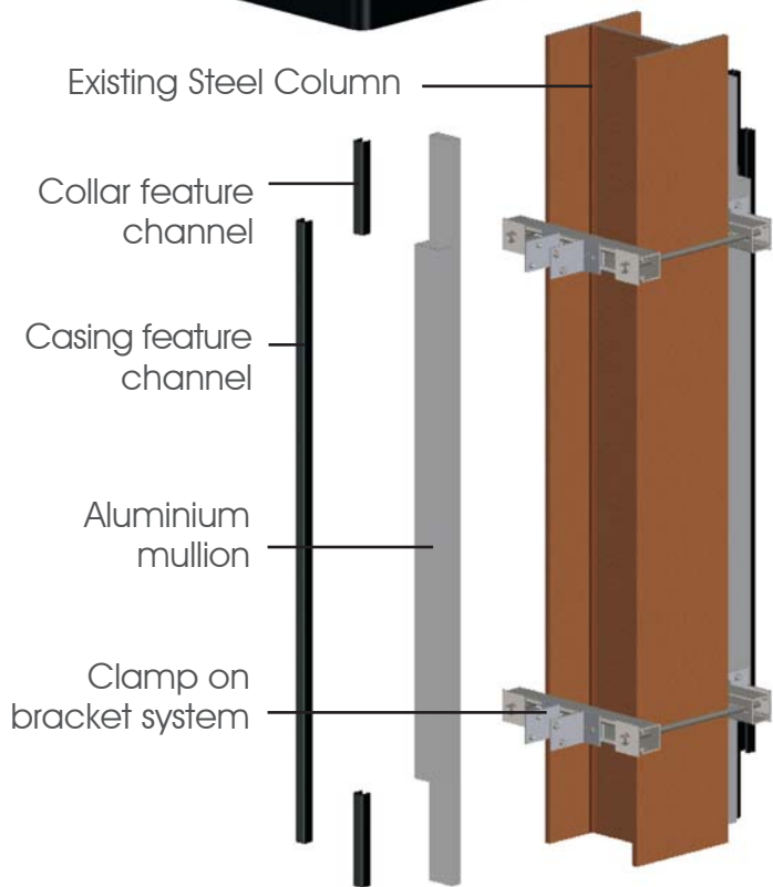
1st Fix Casing
