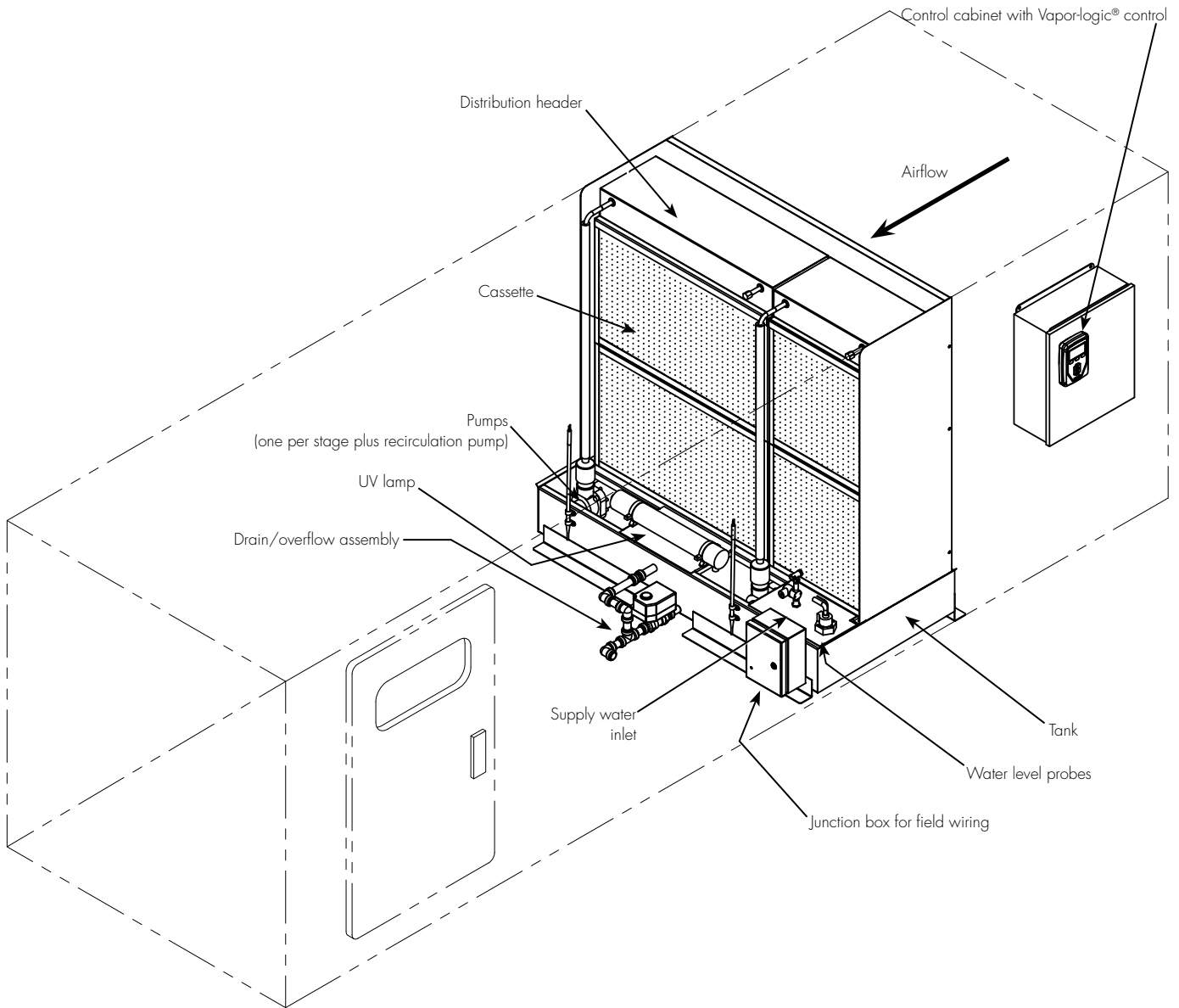
FIGURE 4-1: DRISTEEM WETTED MEDIA SYSTEM OVERVIEW
