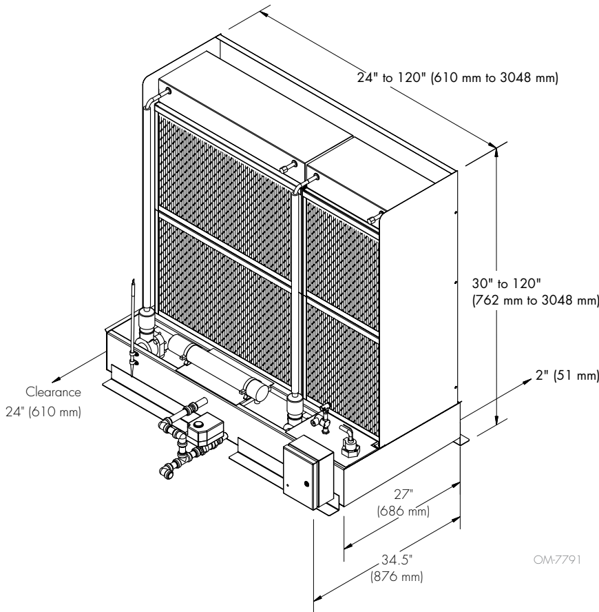
FIGURE 6-2: DRISTEEM WETTED MEDIA SYSTEM DIMENSIONS AND CLEARANCES
