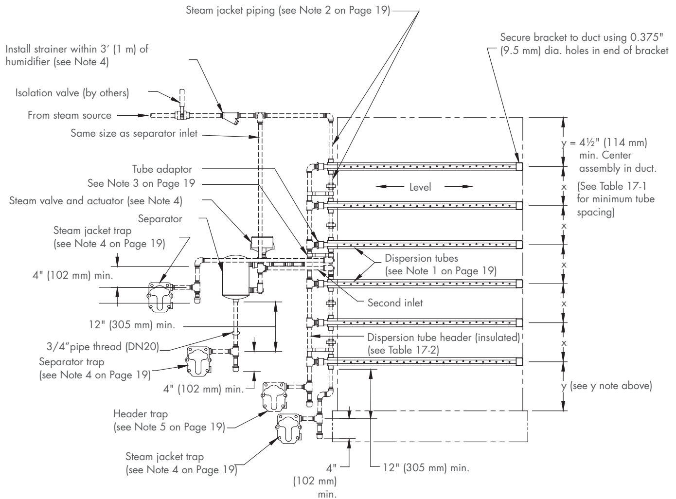
FIGURE 20-1: MULTIPLE-TUBE HUMIDIFIER WITH TOTAL TUBE LENGTH GREATER THAN 45' (13.7 M) IN AN AHU
