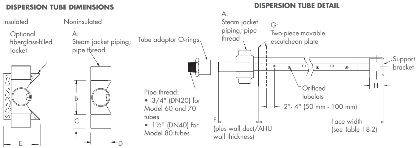
FIGURE 17-1: MULTIPLE-TUBE HUMIDIFIER DISPERSION TUBE DIMENSIONS
