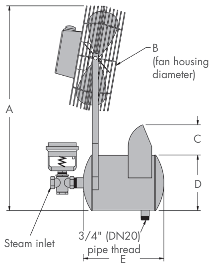
FIGURE 25-1: AREA-TYPE HUMIDIFIER
