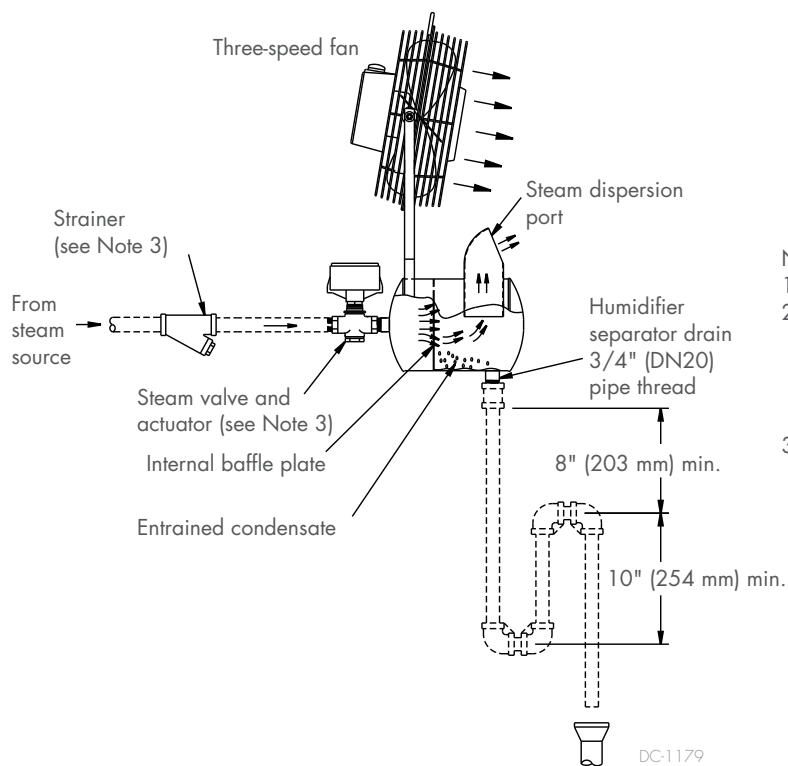
FIGURE 23-2: AREA-TYPE HUMIDIFIER COMPONENTS AND INSTALLATION OVERVIEW
