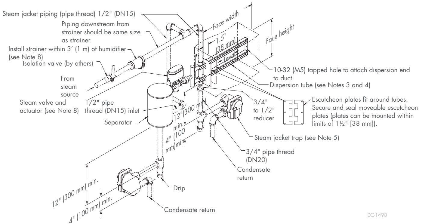
FIGURE 14-1: MINI-BANK HUMIDIFIER INSTALLED IN A DUCT WITH HORIZONTAL AIRFLOW
