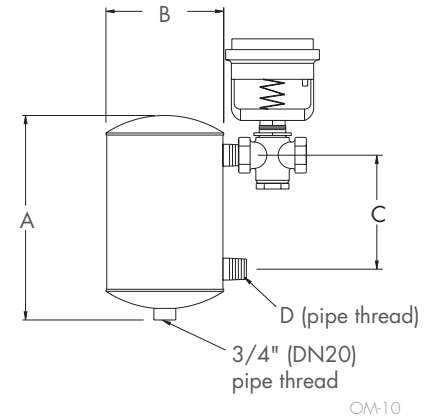
FIGURE 18-1: MULTIPLE-TUBE HUMIDIFIER SEPARATOR DIMENSIONS
