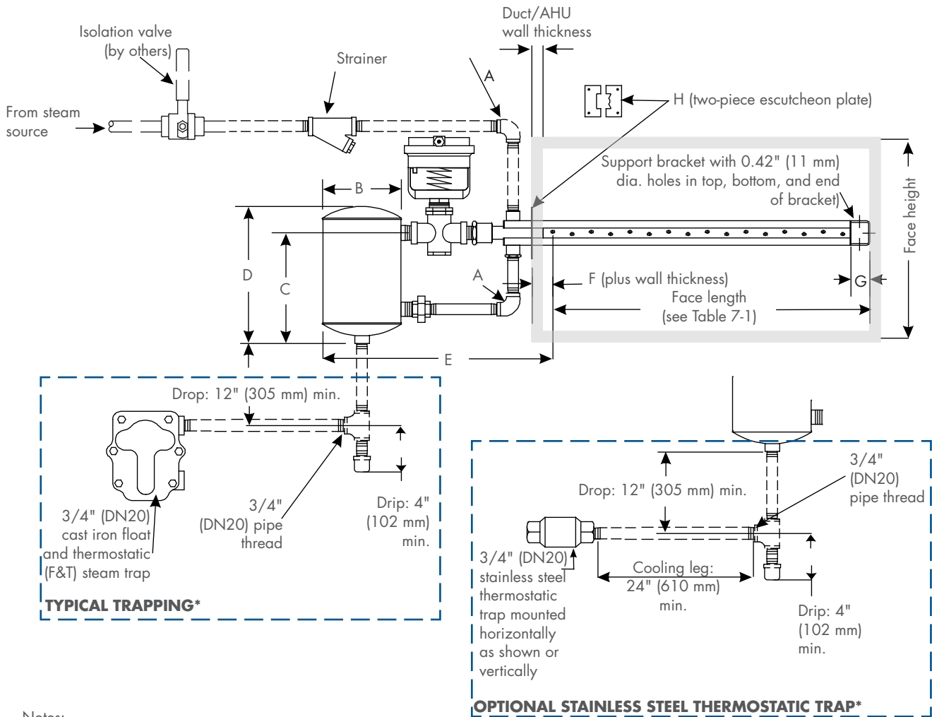
FIGURE 8-1: SINGLE-TUBE HUMIDIFIER DIMENSIONS
