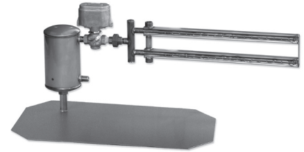
FIGURE 12-1: MINI-BANK HUMIDIFIER
