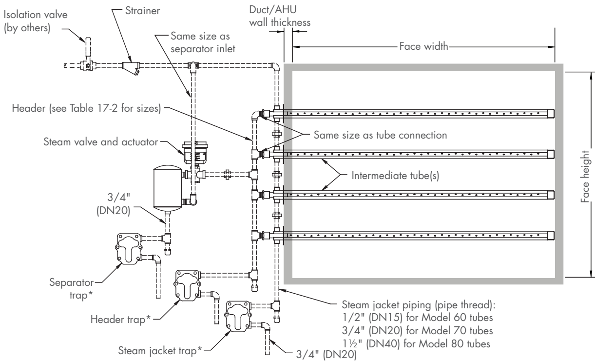
FIGURE 16-2: MULTIPLE-TUBE HUMIDIFIER
