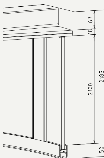
Body – glass ceiling without frame
