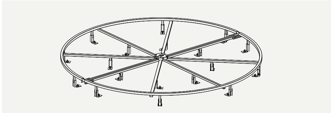
Floor element without stainless steel plate for sealing
