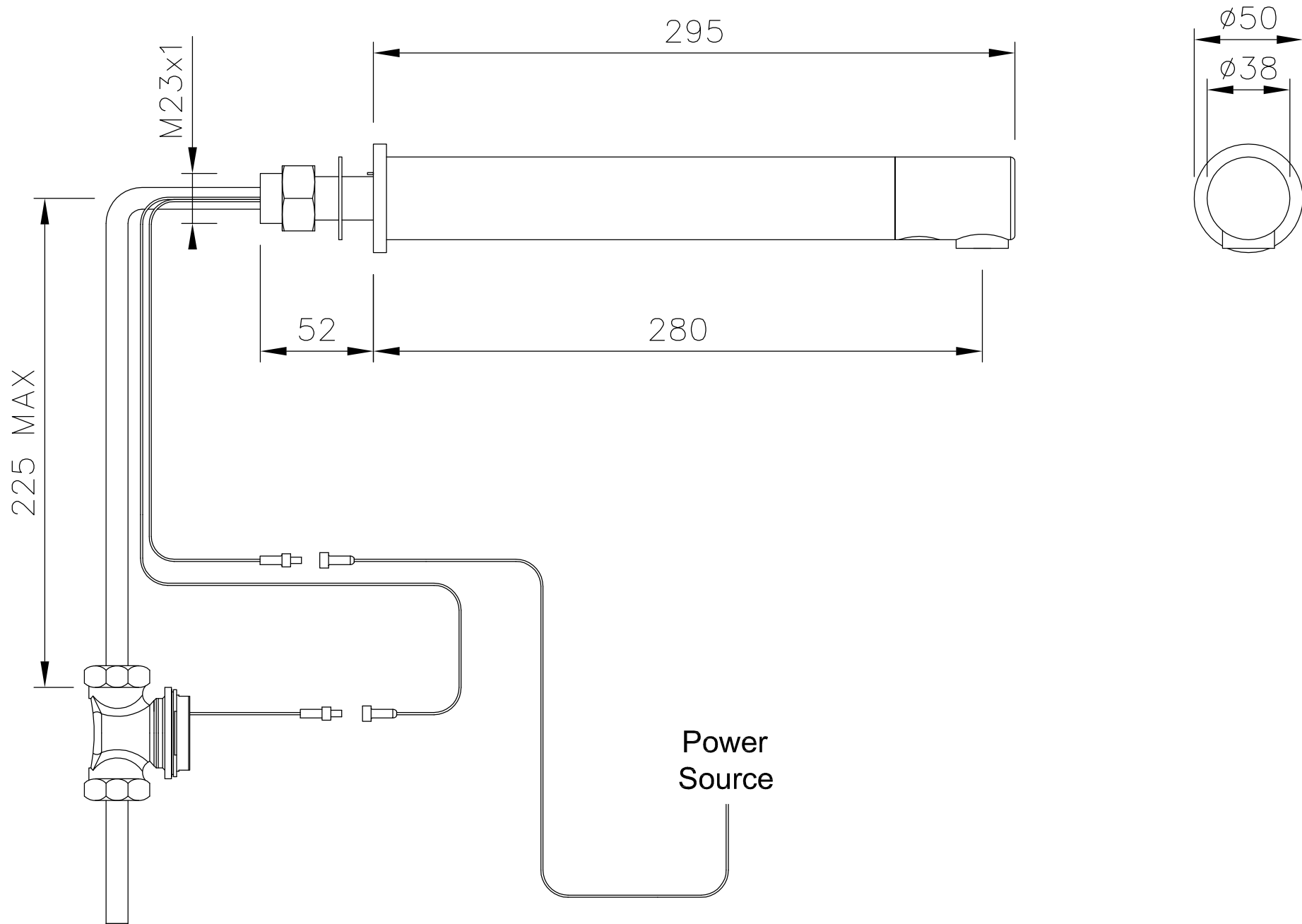
BELL-CHEM PRODUCTS COMPANY DOLPHIN BLUE PANEL MOUNTED ELECTRONIC INFRARED TAP DBXL400 / DBXL425
