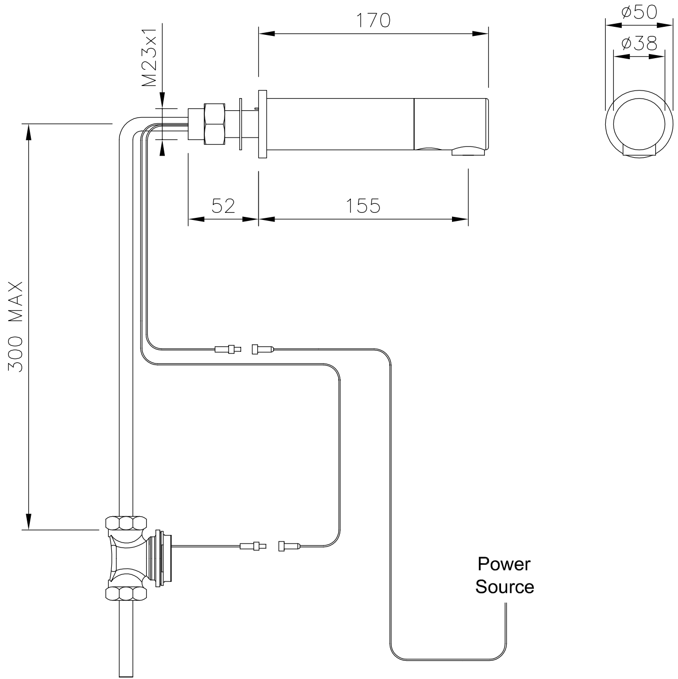
BELL-CHEM PRODUCTS COMPANY DOLPHIN BLUE PANEL MOUNTED ELECTRONIC INFRARED TAP DB400 / DB425
