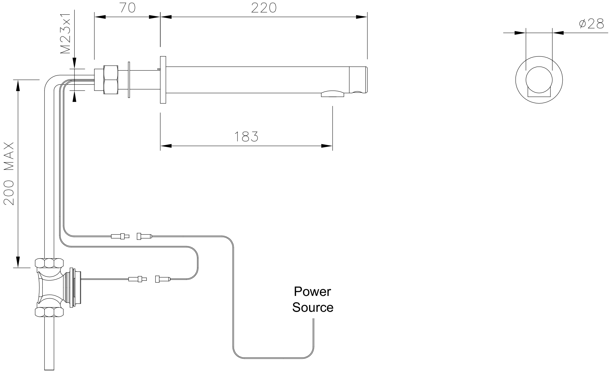
BELL-CHEM PRODUCTS COMPANY DOLPHIN BLUE PANEL MOUNTED ELECTRONIC INFRARED TAP DB1400 / DB1425
