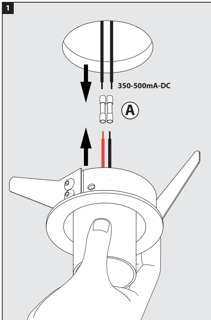
ELECTRICAL CONNECTION
