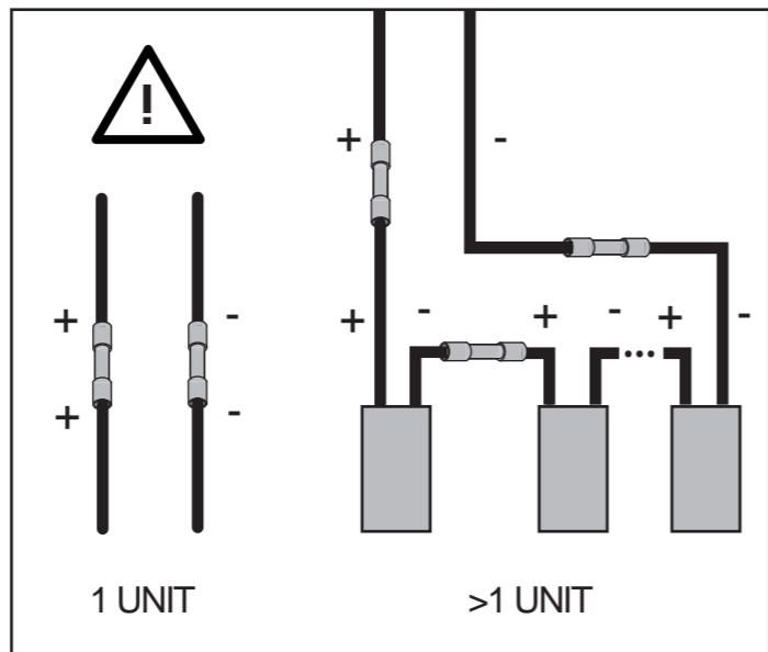
ELECTRICAL CONNECTION
