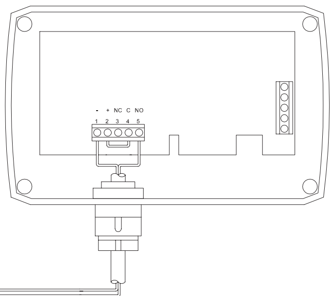
AlertMaxx High Level Alarm (DMS-269/270)
