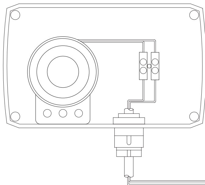
AwareMaxx Remote Buzzer Box (DMS-297)
