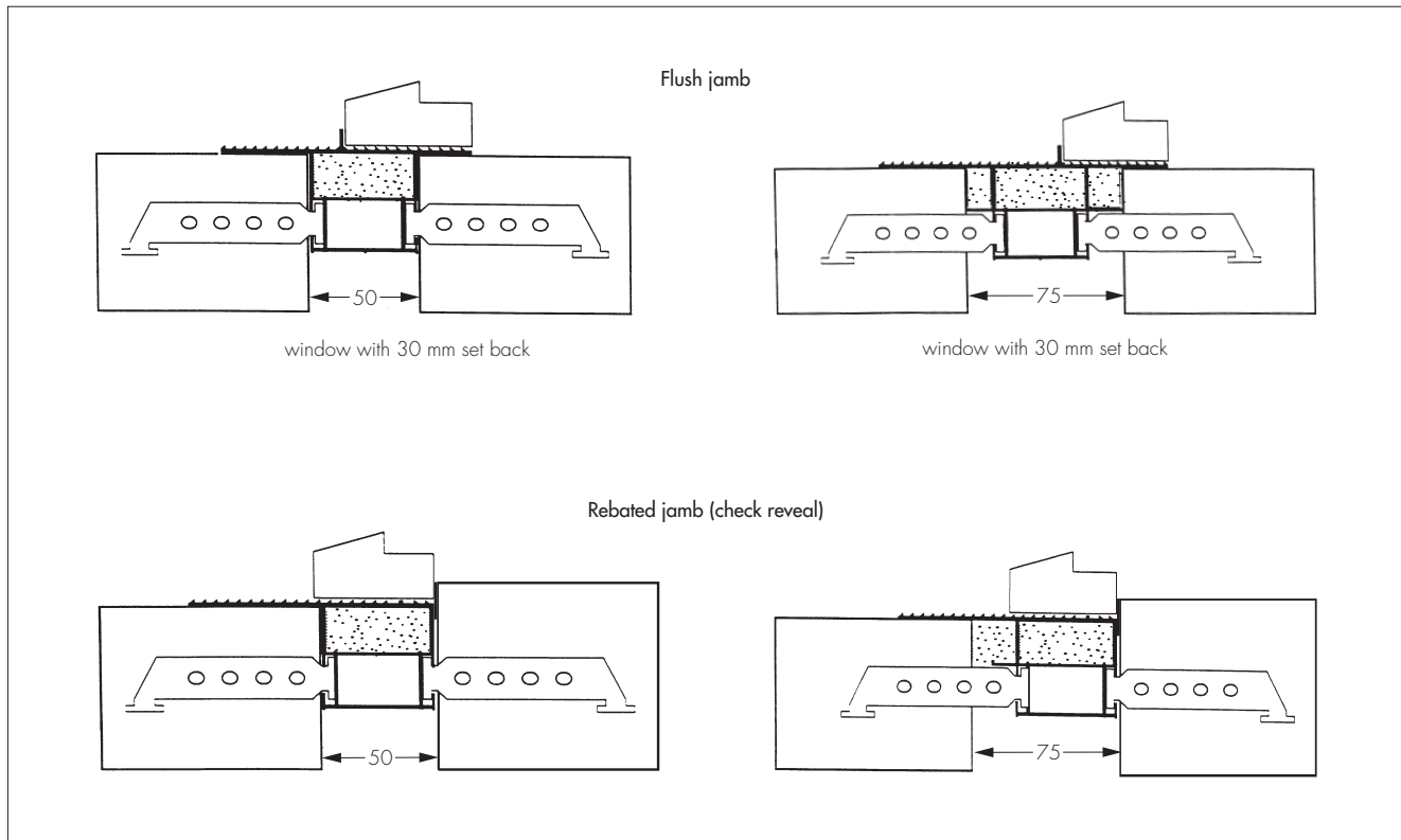
Figure 3 Typical jamb details (all dimensions in mm)
