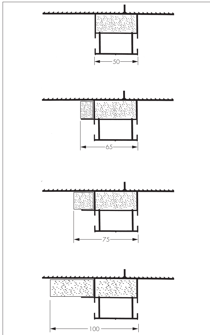
Figure 1 Closers for flush jamb (all dimensions in mm) (example sizes)
