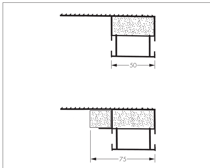
Figure 2 Closers for check reveal (all dimensions in mm) (example sizes)
