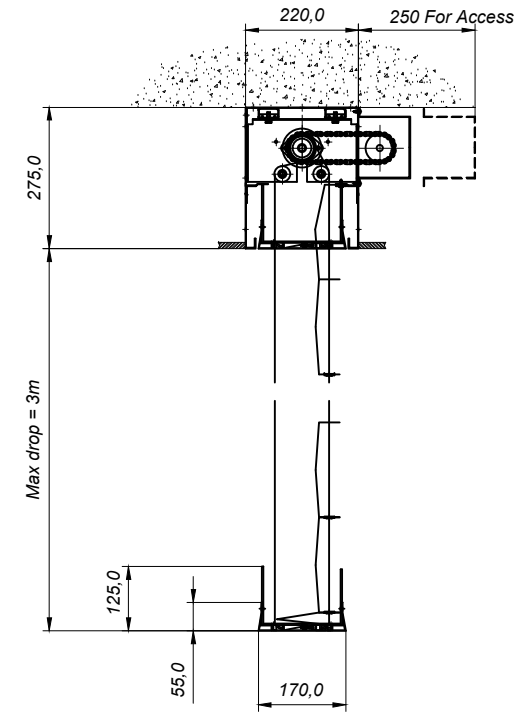
Section Through Curtain
