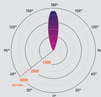
4000K 26° Additional diagrams available at collingwoodlighting.com
