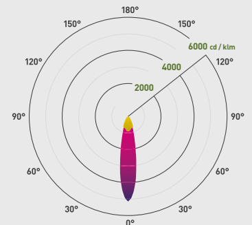
4000K 20° / 4000K 70° Additional diagrams available at collingwoodlighting.com
