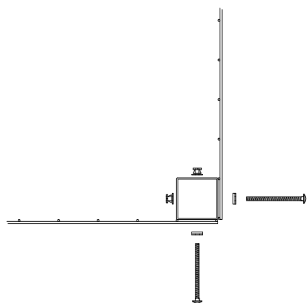
CORNER PLAN 80 x 80 post 1:10
