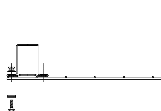
END PLAN 80 x 60 post 1:10
