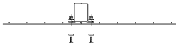
IN-LINE PLAN 80 x 60 post 1:10
