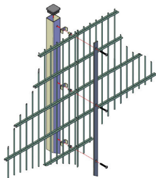
POST FIXING SCHEMATIC (ABOVE)
