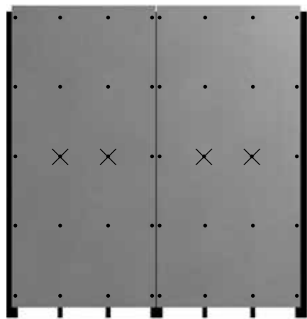
Example: Vertically mounted boards with two intermediate steel profiles
