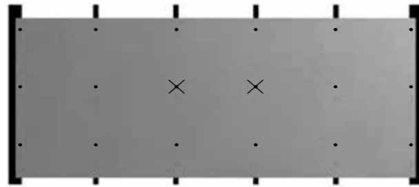
Example: Horizontally mounted boards with four intermediate steel profiles
