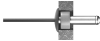
X : Fixing position hole diameter \varnothing 9 mm. Insert a Cembrit Fixing Sleeve in the hole before the rivet is fixed.
