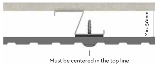
Fig. 2. Cembrit Patina Inline installation on the middle profile.
