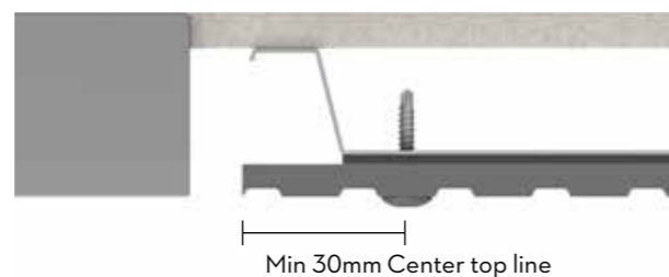
Fig. 4. Cembrit Patina Inline installation on cut to size board.
