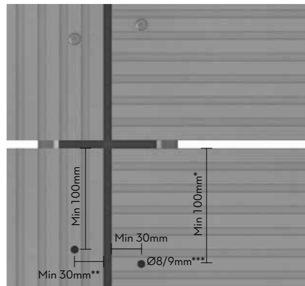
Fig. 3. Cembrit Patina Inline edge distances. Note! Min distance and/or the nearest following top line. ***9mm drill bit for rivet and a 8mm drill bit for screws.
