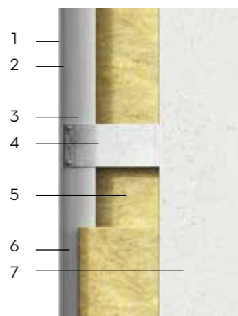
Joint profile
