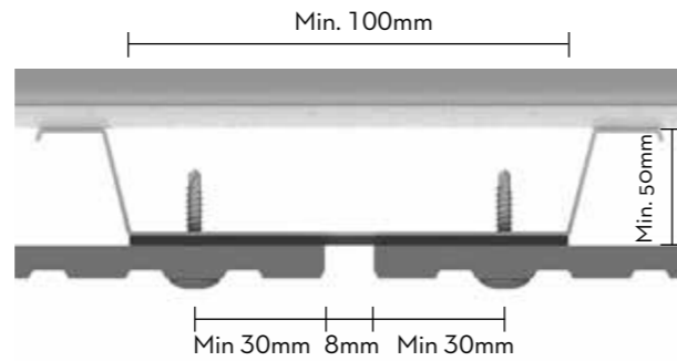
Fig. 1. Cembrit Patina Inline installation on profile behind joint.
