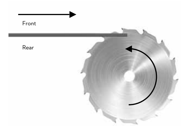
When using a table saw, place the board with the face uppermost on the table and cut from the rear of the board.
