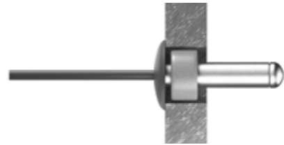
X : Fixing position hole diameter Ø9 mm. Insert a Cembrit Fixing Sleeve in the hole before the rivet is fixed.
