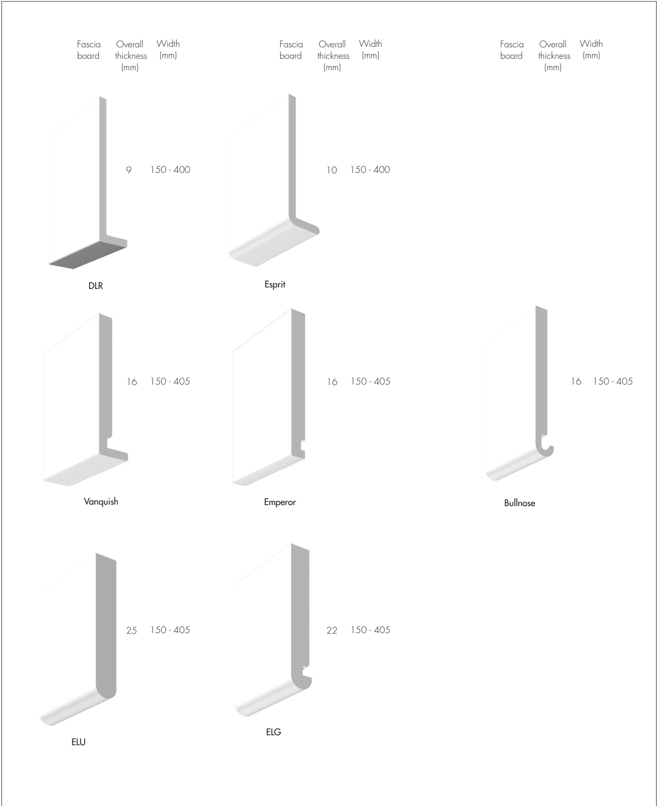
Figure 1 Fascia/Barge boards
