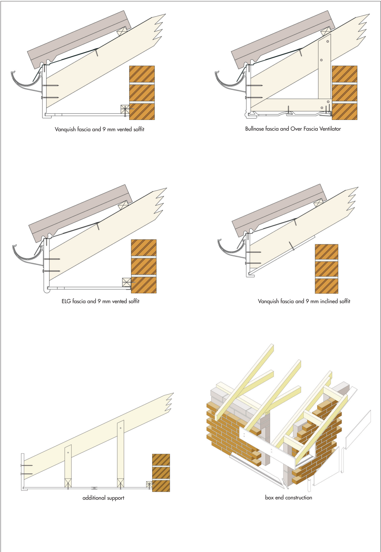
Figure 4 Typical fascia and soffit installation details
