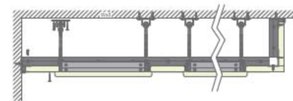
Plan view of RPM wall system
