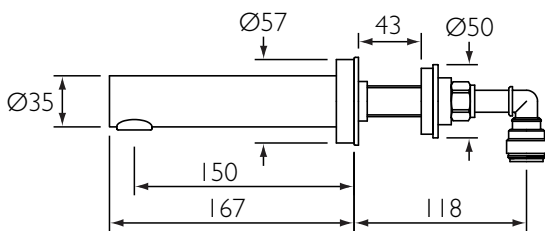
AWS150S-CP
