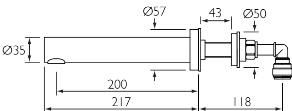
AWS200L-CP
