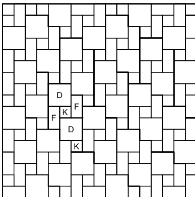
Pattern No. 5 Repeatable Pattern Area = 1.31 sq.m. Quantities per Repeatable Pattern (D) 600 x 600mm - 2 No. (F) 600 x 300mm - 2 No. (K) 300 x 300mm - 2 No. Dimensions are approximate and include a 10mm joint.
