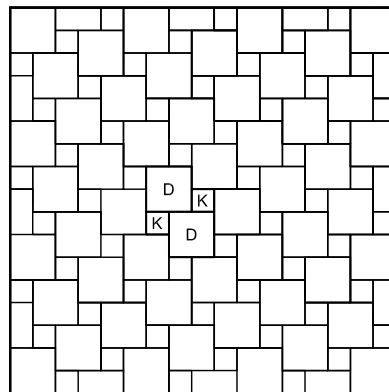
Pattern No. 6 Repeatable Pattern Area = 0.94 sq.m. Quantities per Repeatable Pattern (D) 600 x 600mm - 2 No. (K) 300 x 300mm - 2 No. Dimensions are approximate and include a 10mm joint.
