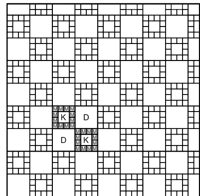
Pattern No. 9 Repeatable Pattern Area = 1.44 sq.m. Quantities per Repeatable Pattern (D) 600 x 600mm - 2 No. (K) 300 x 300mm - 2 No. (M) 150 x 150mm - 24 No. (M) 150x150mm can be achieved with the Patlo Square or Rosett ranges Dimensions are approximate and include a 10mm joint.
