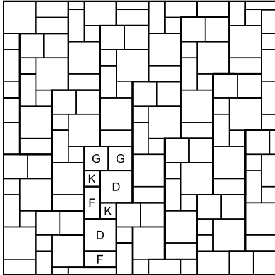
Pattern No. 11 Repeatable Pattern Area = 1.74 sq.m. Quantities per Repeatable Pattern (D) 600 x 600mm - 2 No. (K) 300x300mm - 2 No. (F) 600 x 300mm - 2 No. (G) 450 x 450mm - 2 No. Dimensions are approximate and include a 10mm joint.
