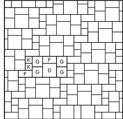
Pattern No. 34 Repeatable Pattern Area = 1.79 sq.m. Quantities per Repeatable Pattern (D) 600 x 600mm - 1 No. (K) 300x300mm - 2 No. (F) 600 x 300mm - 2 No. (G) 450 x 450mm - 4 No. Dimensions are approximate and include a 10mm joint.
