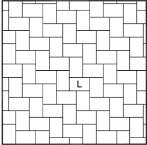
Pattern LU.1 Herringbone - Large 34 No. - Large 210x140mm per sq.m.
