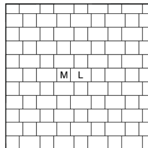
Pattern LU.37 2 Size Stretcher - M & L 21 No. - Medium 140x140mm per sq.m. 21 No. - Large 210x140mm per sq.m.
