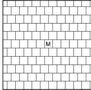
Pattern LU.4 Stretcher Course - Medium 51 No. - Medium 140x140mm per sq.m.
