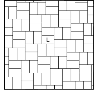
Pattern LU.8 Basket Weave - Large 34 No. - Large 210x140mm per sq.m.
