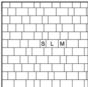
Pattern LU.33 3 Size Random Stretcher 2 6 No. - Small 105x140mm per sq.m. 12 No. - Medium 140x140mm per sq.m. 24 No. - Large 210x140mm per sq.m.
