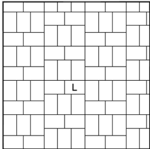
Pattern LU.10 Five Block Cluster - Large 34 No. - Large 210x140mm per sq.m. Recommended for patios only
