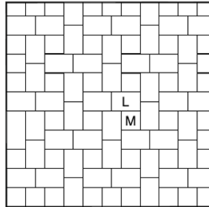
Pattern LU.13 Victorian Weave - M & L 13 No. - Medium 140x140mm per sq.m. 26 No. - Large 210x140mm per sq.m.
