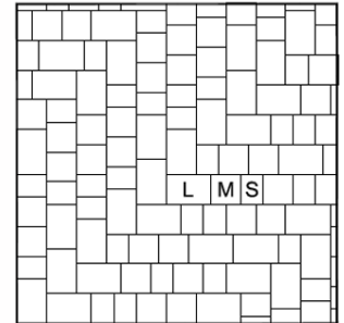
Pattern LU.29 3 Size Random Herringbone 16 No. - Small 105x140mm per sq.m. 16 No. - Medium 140x140mm per sq.m. 16 No. - Large 210x140mm per sq.m.
