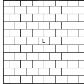
Pattern LU.5 Stretcher Course - Large 34 No. - Large 210x140mm per sq.m.
