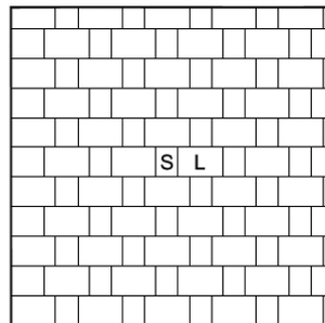
Pattern LU.34 2 Size Stretcher - S & L 23 No. - Small 105x140mm per sq.m. 23 No. - Large 210x140mm per sq.m.
