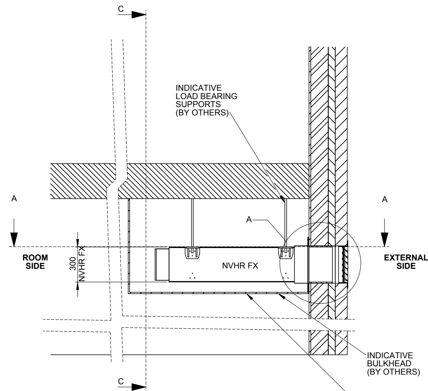
SECTION B-B
