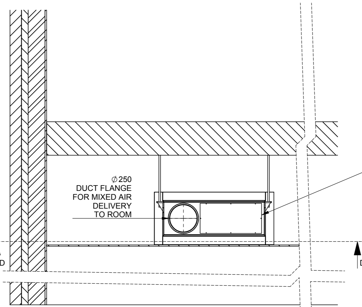
SECTION C-C
