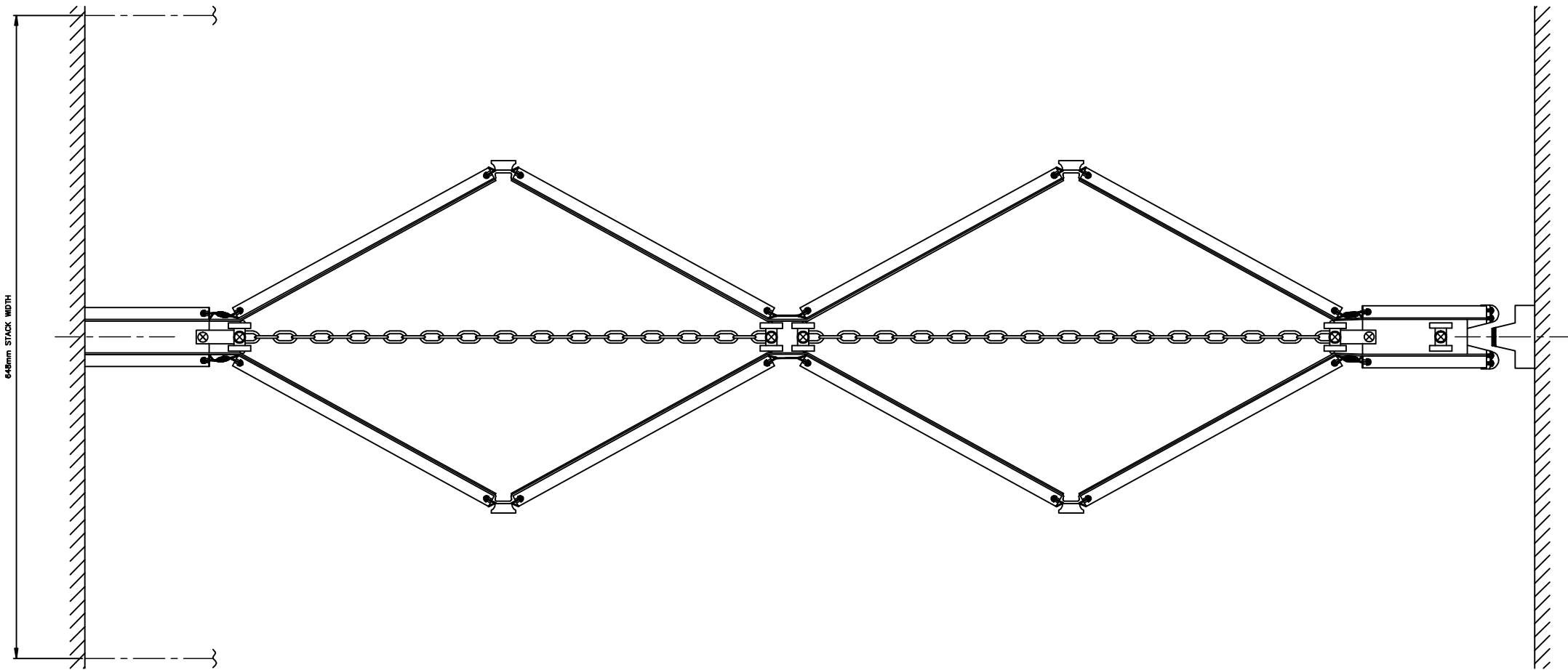
BECKER (SLIDING PARTITIONS) LTD. DUPLO 122 Horizontal section
