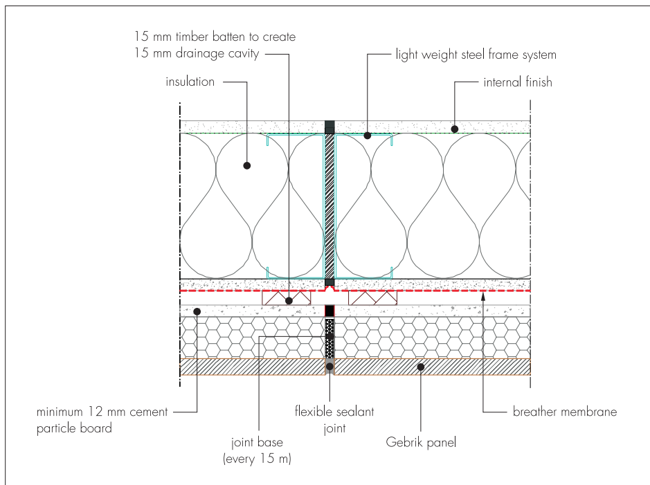
Figure 9 Movement joint
