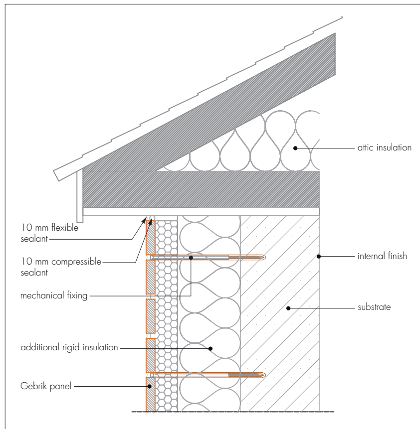
Figure 10 Typical roof eaves details
