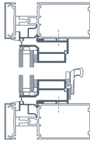
GLASSvent™ Window for Curtain Wall
