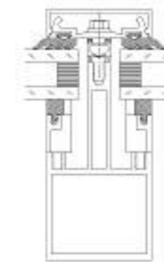
ACS 20CW Vertical Mullion
