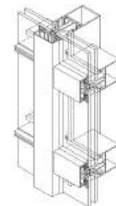
ACS 20CW Facecap Installation Assembly Detail
