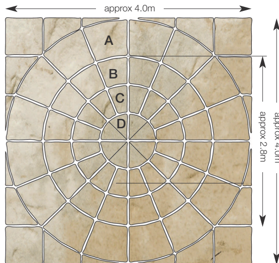
4m \varnothing circle with 4m 2 squaring off kit
