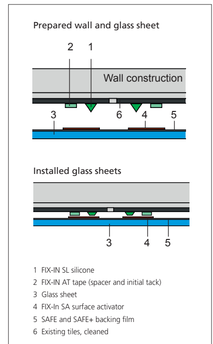
GLASS WITH SAFE AND SAFE+ BACKING FILM
