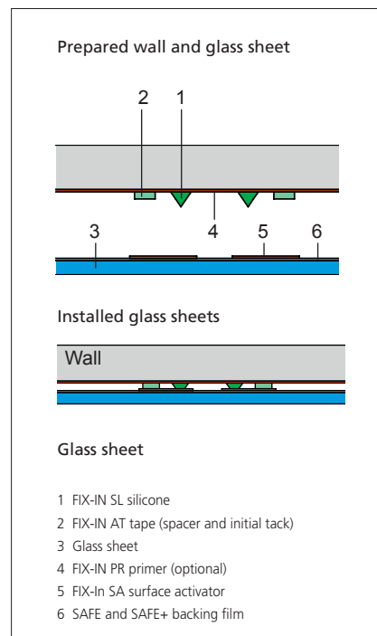
GLASS WITH SAFE AND SAFE+ BACKING FILM
