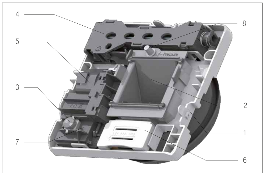
Presented version : BXC with presence detection and humidity sensitive sensor
