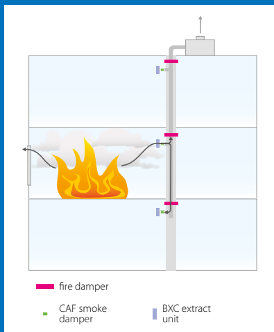
CAF - Smoke damper
