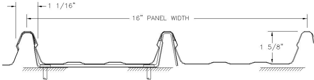
Figure 3.1 - Profile: As-installed view shown.
