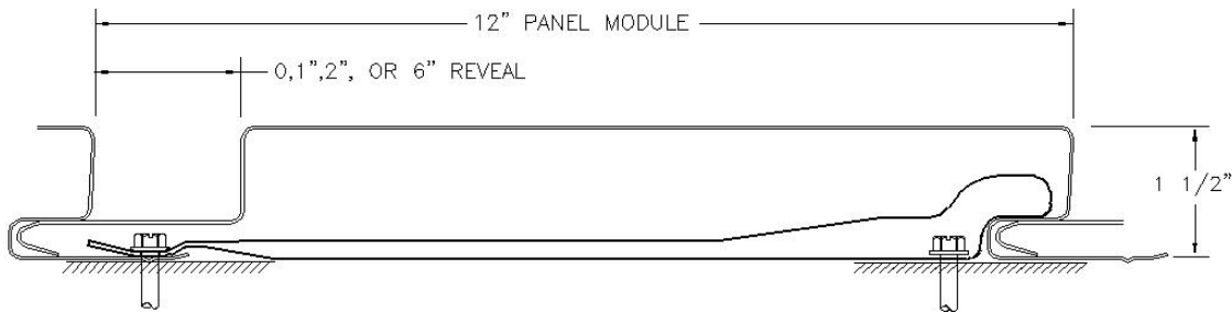
Figure 5.1 - Profile: As installed view shown, with optional clip.
