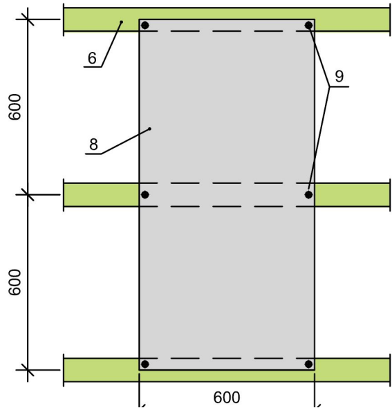
Panel 600 x 1200mm, fixed with 6 screws
