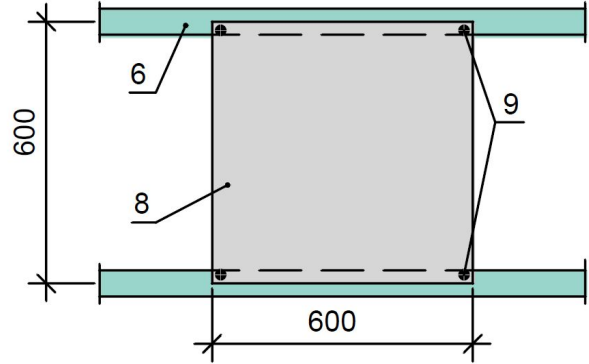
Panel 600 x 600mm, fixed with 4 screws
