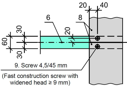
Panel 600 x 1200mm, fixed with 8 screws
