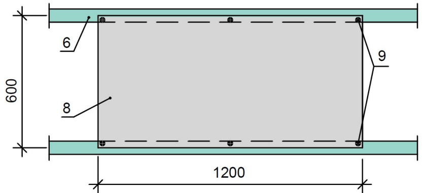
Panel 600 x 1200mm, fixed with 6 screws longitudinally on laths
