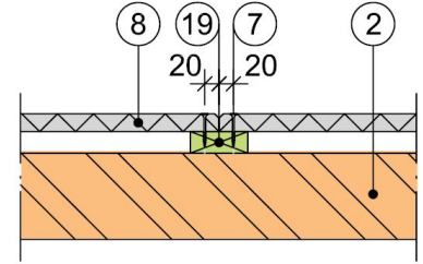
Wood lathing fastening on to a load-bearing wall structure
