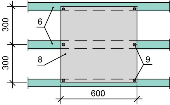
Panel 600 x 600mm, fixed with 6 screws
