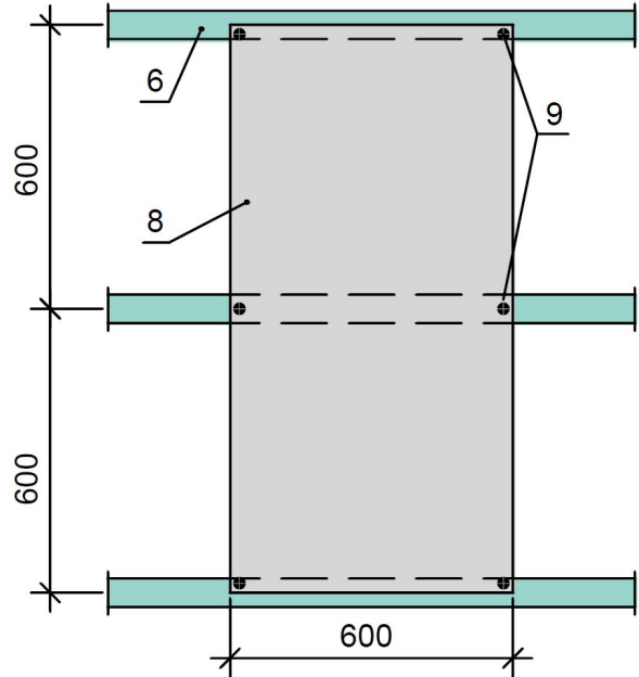
Panel 600 x 1200mm, fixed with 6 screws
