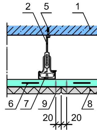
Joint between end edges.
