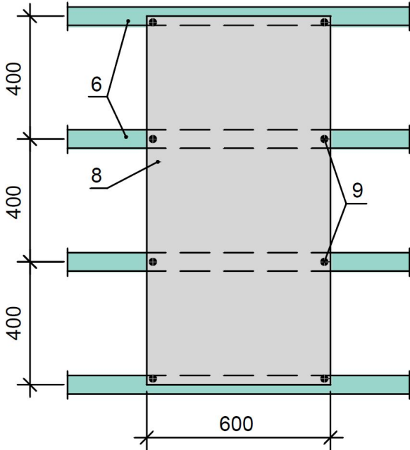
Panel 600 x 1200mm, fixed with 8 screws
