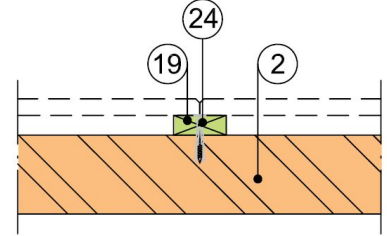
Wood lathing fastening on to a load-bearing wall structure
