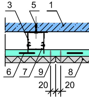
Joint between end edges.
