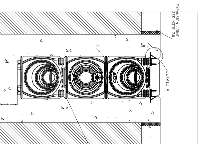
ACO QMAX 225 & 350 ACCESS, OUTLET/INLET AND SILT CHAMBER WITH SLOTTED COVER AND FRAME
