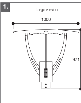
Dimensions & Mounting 60mm/114mm spigot Mounting height: 4m – 6m
