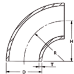
Welded 45° & 90° elbows (radius 1.5D)
