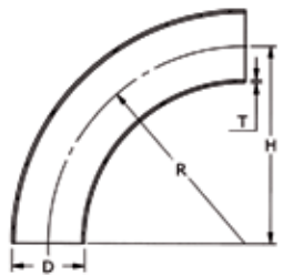
Welded 45° & 90° elbows (radius D+100)
