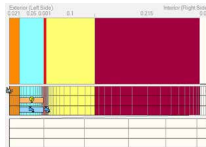
Rainscreen Brick Wall with external PIR/Rockwool
